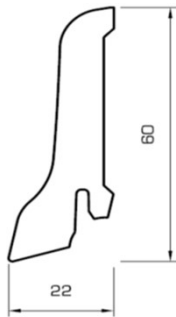
MFS6022 - 60 x 22mm
