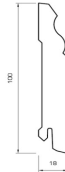
MFS100C - 100 x 18mm Classic
